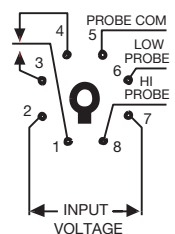
PIN CONFIGURATION
